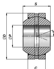
TYPE FO...2RS
