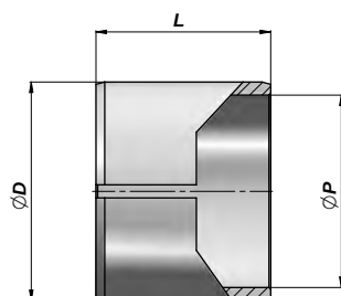
TYPE ADU
