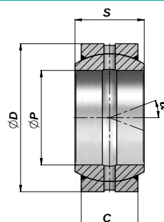
TYPE D0...2RS
